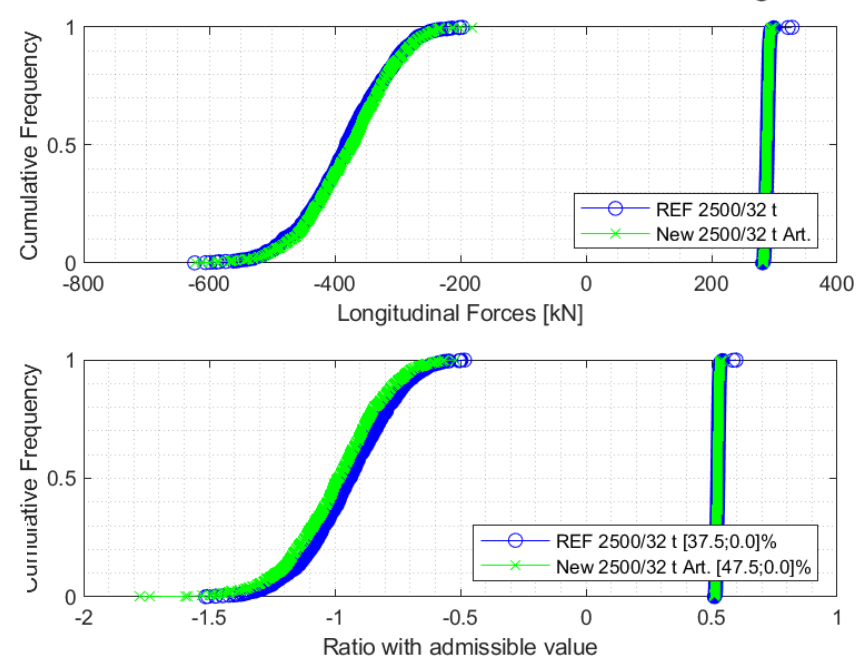
Ref and new trains 2500 t with Articulated wagons
