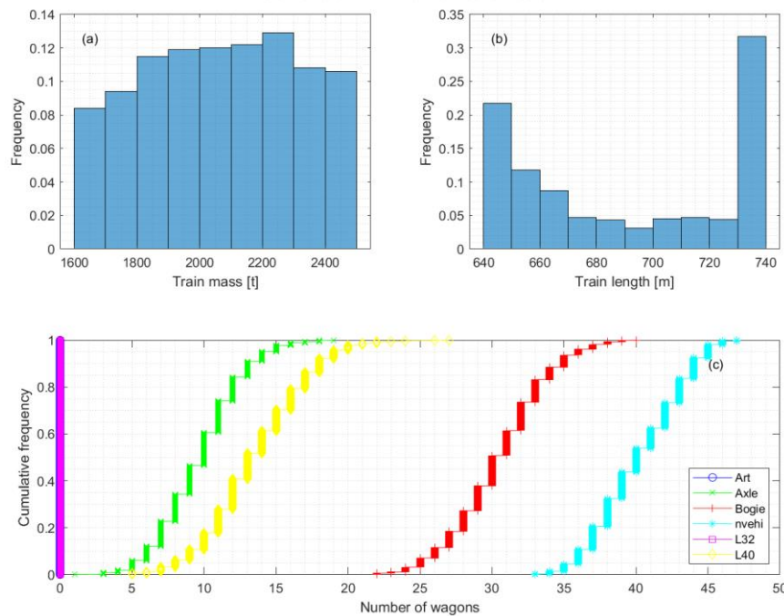
Statistics REF1 trains 1600-2500
