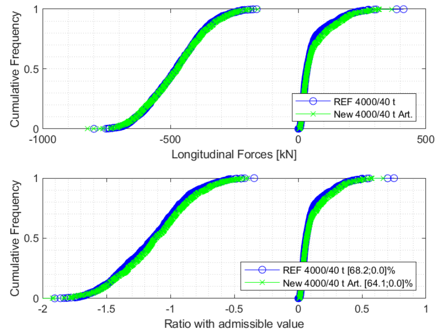
Ref and new trains 4000 t with Articulated wagons EB
